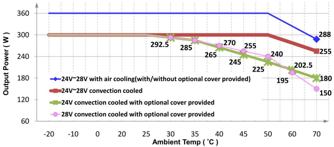
Derating curves of 24V~28V output (MPM-U305, MPM-U305-C)
