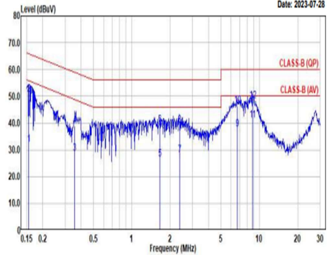
EMI: FCC "B" (Conduction)
