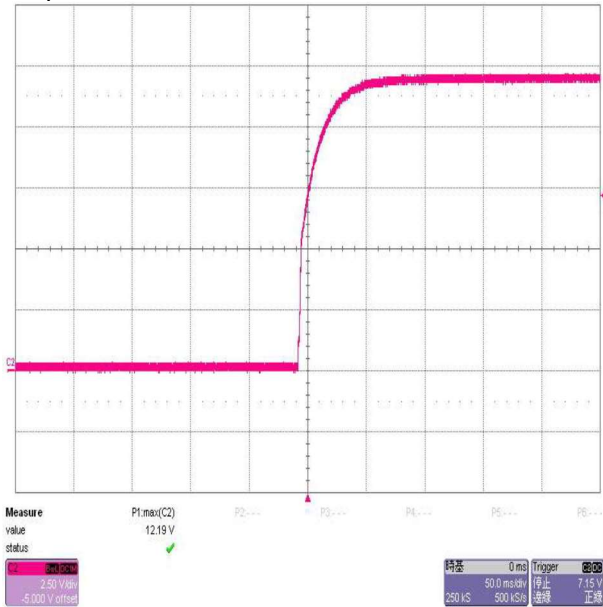
Output turn on rated load
