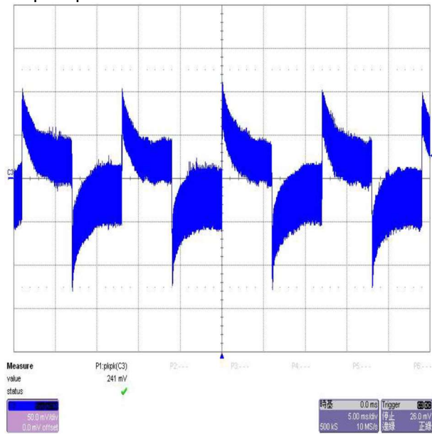
Step response 20%~100% of rated load
