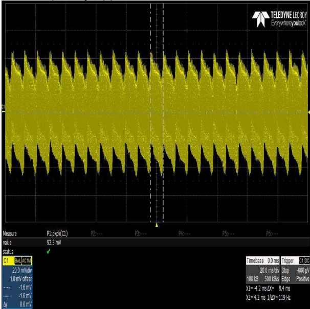
Line frequency ripple rated load
