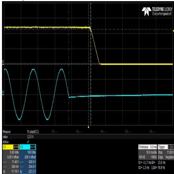
Hold up time rated load
