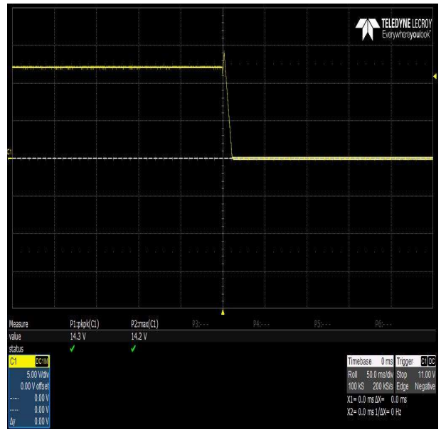
OVP 60% of rated load
