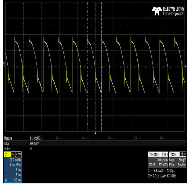
Switching frequency ripple rated load
