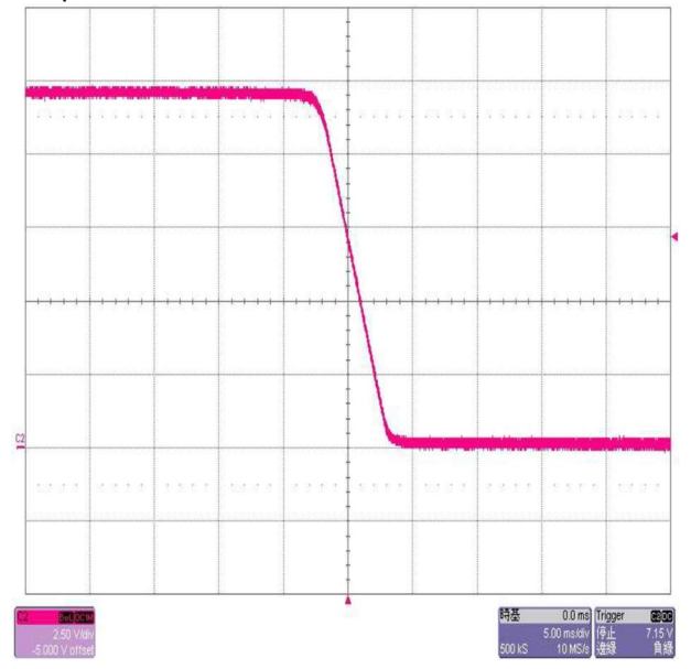
Output turn off rated load
